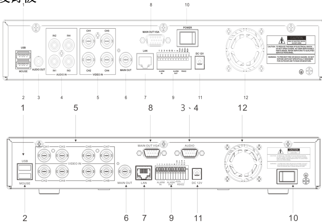
(4-8CH_DVR 後背板圖示)
